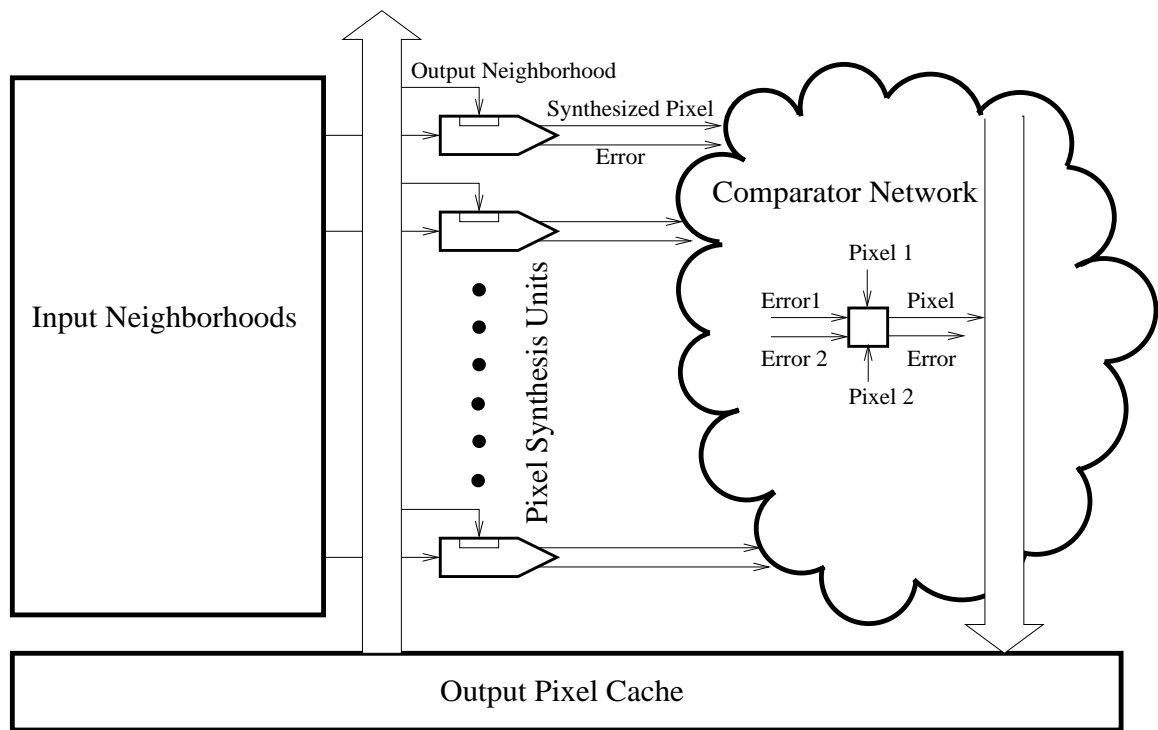
Figure 8.8: Our texture synthesis architecture.
