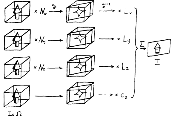
Figure 6: Algorithm for generating a directionally shaded rendering of a volume dataset. During precomputation, volume I_s \Omega is multiplied by orientation field \mathbf{N} . For each view, the extracted slices are multiplied by lighting direction \mathbf{L} .
