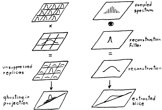
Figure 2: Imperfect reconstruction in the frequency domain produces incompletely suppressed replicas in the spatial domain. These appear in the image as noticeable ghosting.
