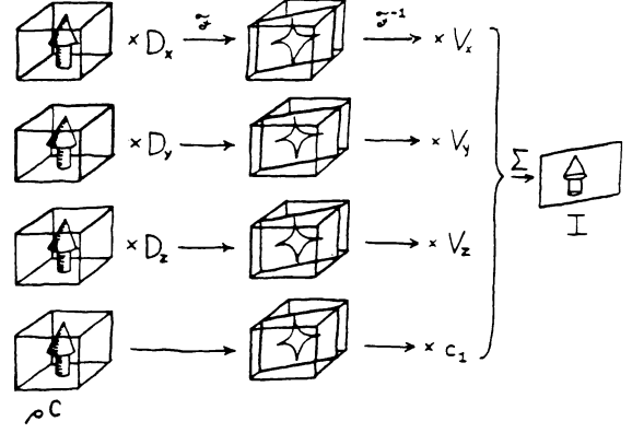
Figure 4: Algorithm for generating a depth cued rendering of a volume dataset. During precomputation, volume \rho C is multiplied by depth operator D . For each view, the extracted slices are multiplied by viewing direction \mathbf{V} .
