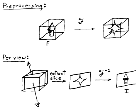
Figure 1: Algorithm for generating an attenuation-only rendering of a volume dataset using the Fourier projection-slice theorem.
