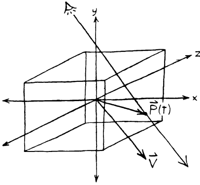
Figure 3: Linear depth cueing for a volume centered at the origin is given by D = m \mathbf{P} + b for constants m and b where \mathbf{P}(t) is position along a viewing ray and \mathbf{V} is the normalized viewing direction.
