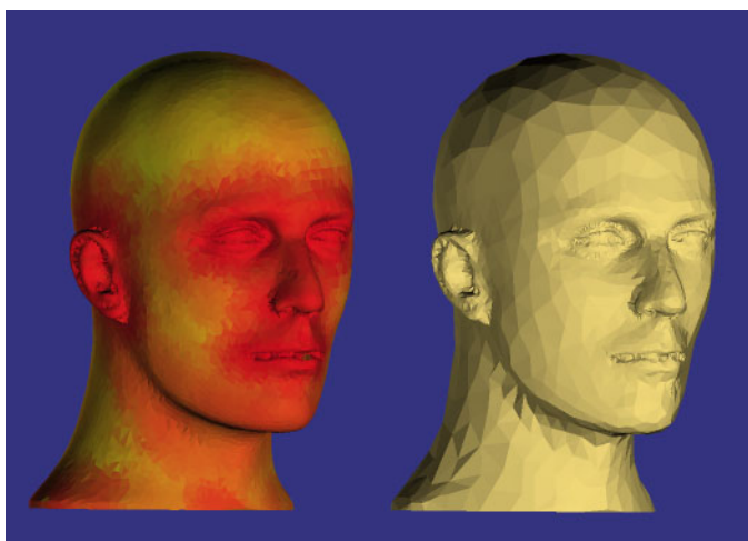
Figure 4. The sampling spacing required to correctly reconstruct a surface is proportional to the distance to the medial axis. On the left is a surface reconstructed from a dense sample. The color represents estimated distance to medial axis—red means close. On the right, we use the estimated distance to thin the data to a .5-sample (meaning that the distance to the nearest sample for any point on the surface is at most half the distance to the medial axis), and then reconstruct. There were about 12K samples on the left and about 3K on the right.
