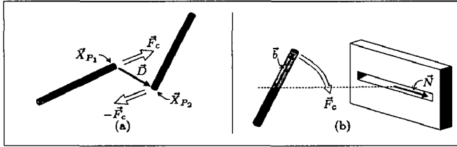
Figure 18: (a) "Point-to-point" constraint. We apply equal-and-opposites to the two constrained points, to cause the deviation function \vec{D}(\mathcal{Y}) = \vec{X}_{P_2}(\mathcal{Y}) - \vec{X}_{P_1}(\mathcal{Y}) to go to 0. (b) "Orientation" constraint. We rotate the body to cause the deviation function \vec{D}(\mathcal{Y}) = \vec{b} \cdot \vec{N} - 1 to go to 0. The constraint torque is given directly by \vec{F}_c ; there is no force due to the constraint.
